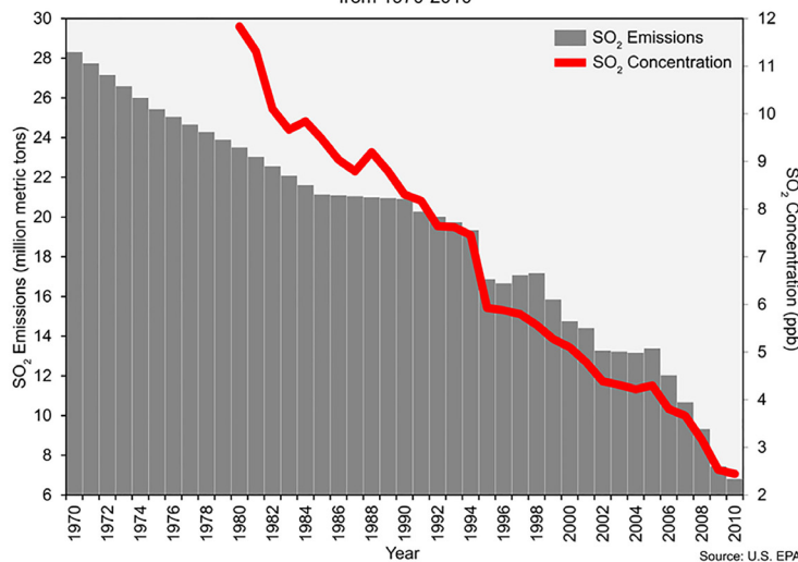
Changes in Emissions and Concentrations of Sulphur Dioxide (SO 2 ) in the United States from 1970-2010
